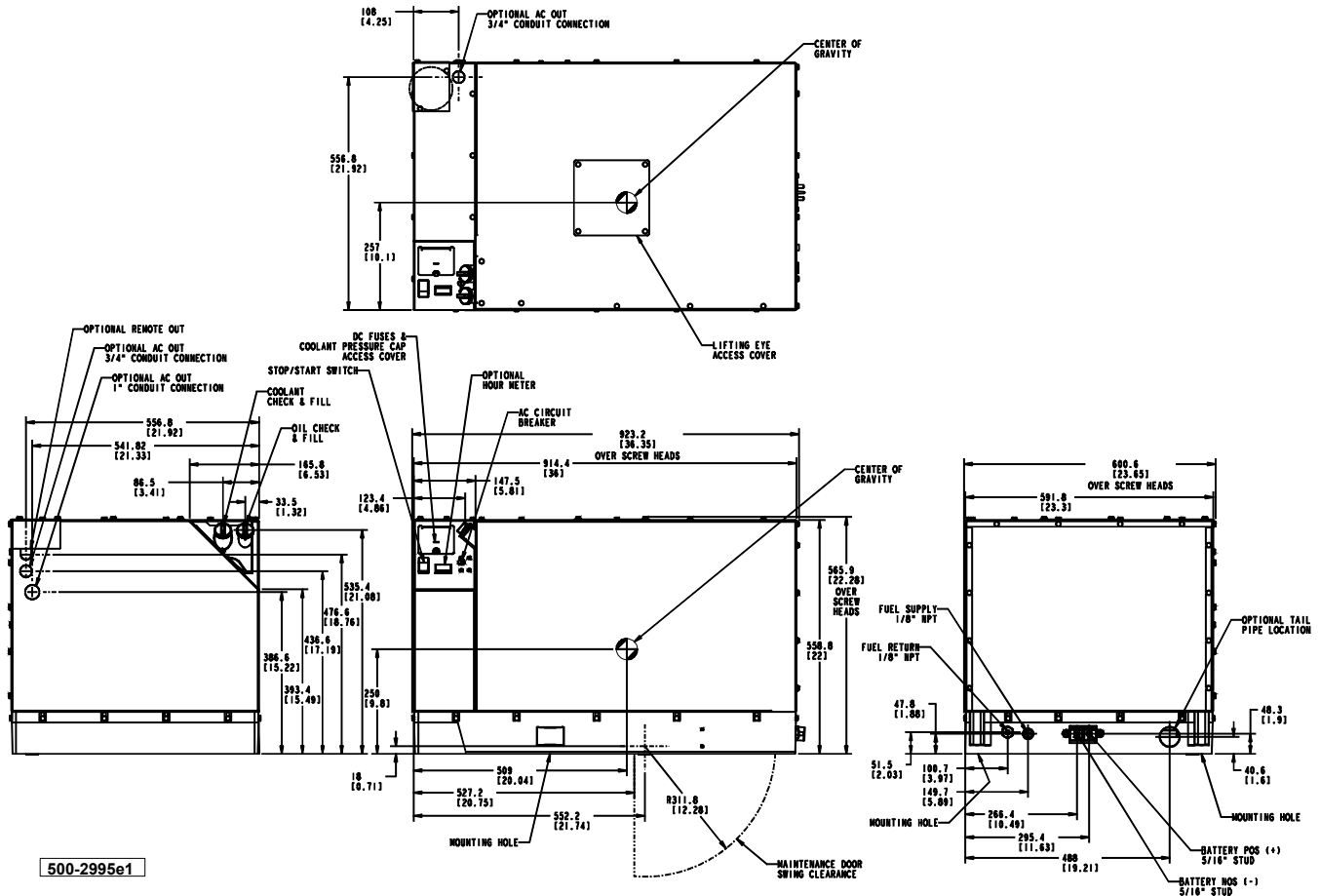
Conventional Compartment Mount
